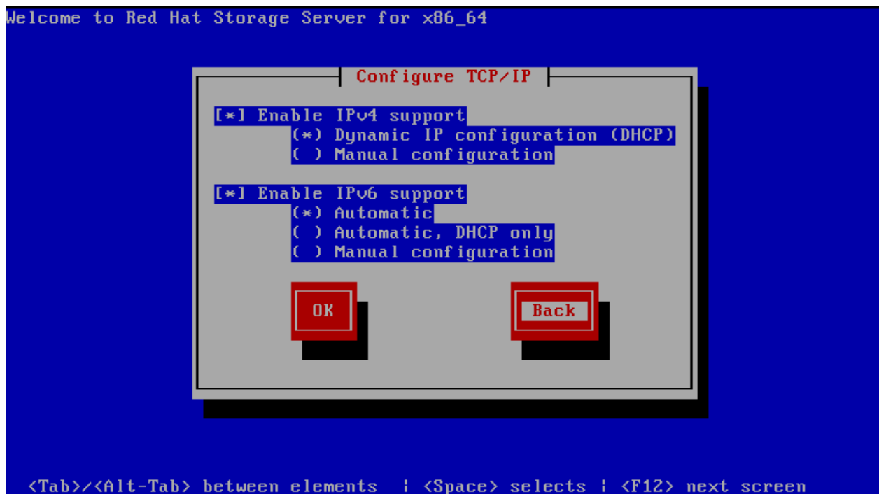
Figure 4.2. Configure TCP/IP
