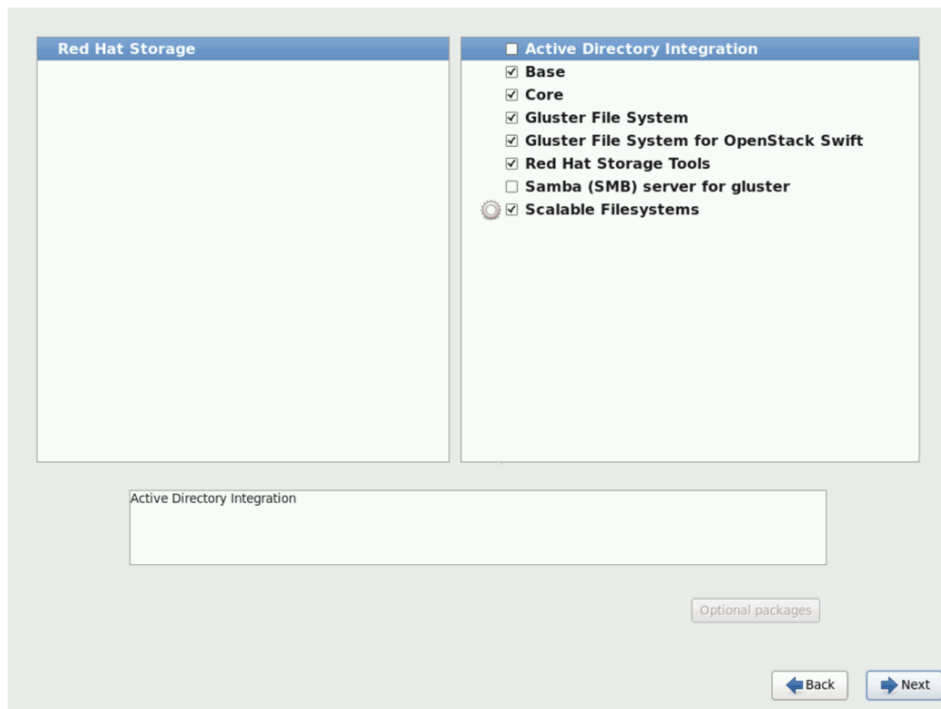
Figure 7.1. Customize Packages
