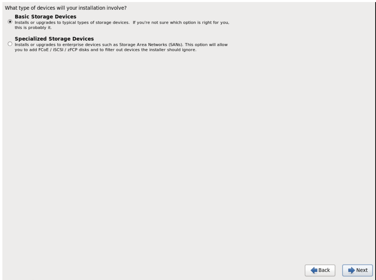
Figure 4.4. Storage Devices
