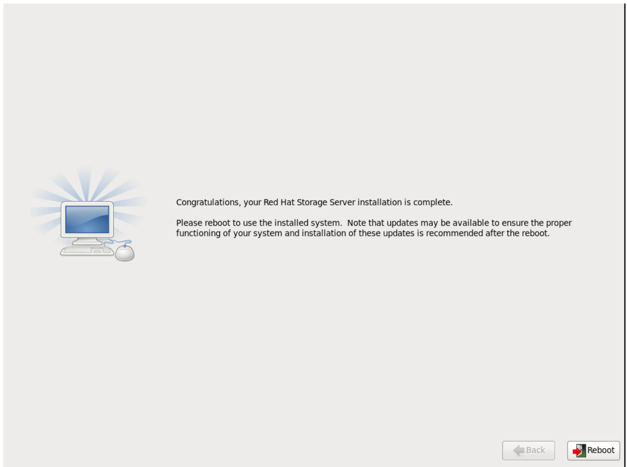
Figure 4.12. Installation Complete
