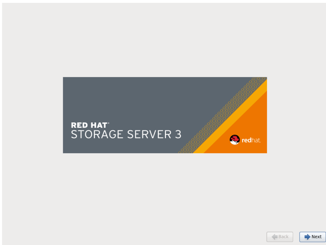
Figure 4.3. Welcome
