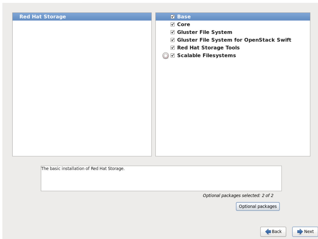
Figure 4.9. Customize Packages
