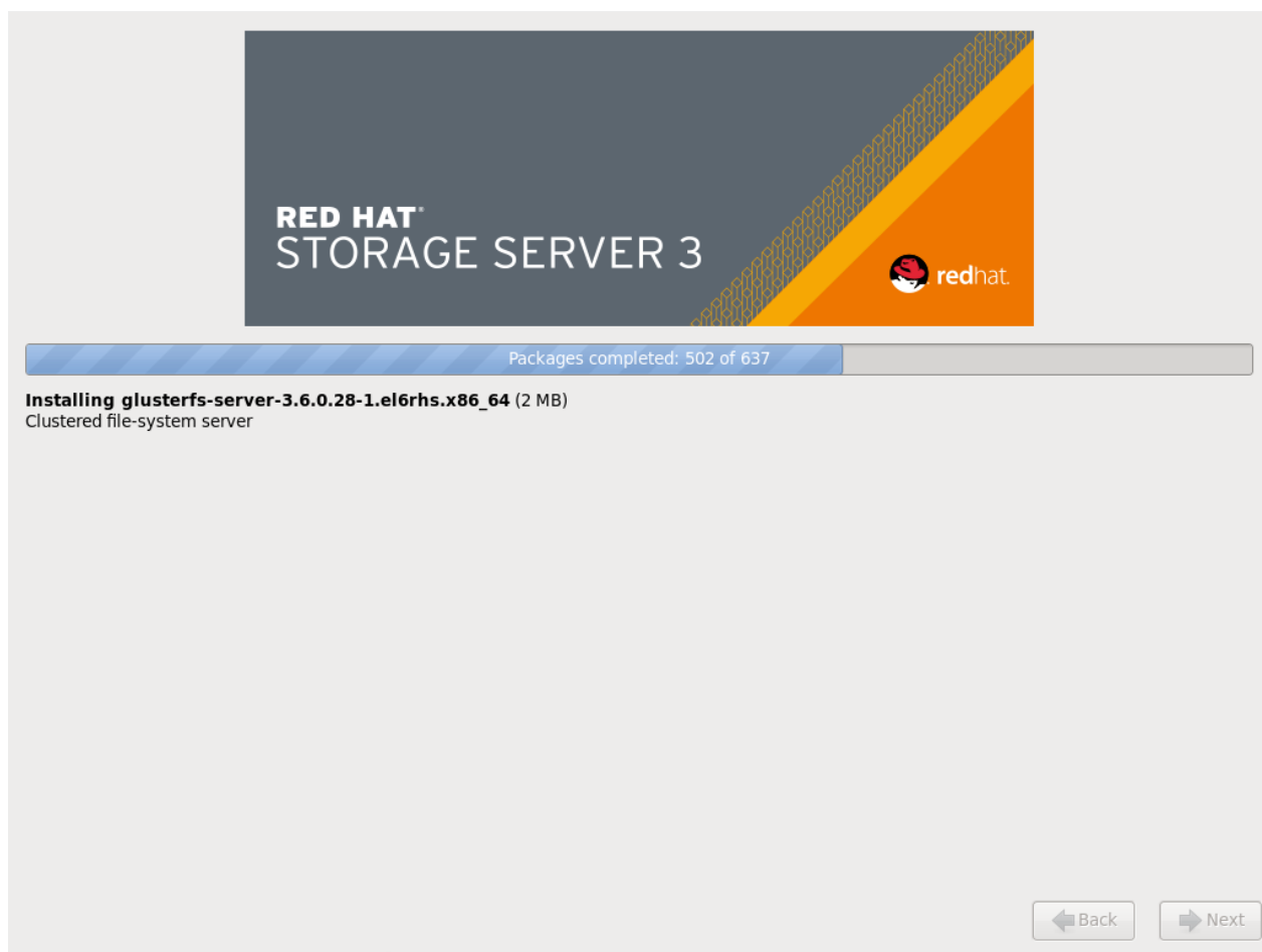
Figure 4.11. Package Installation
