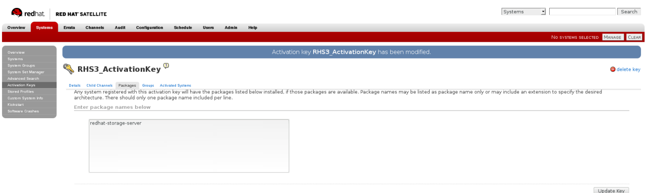
Figure 4.15. Package
