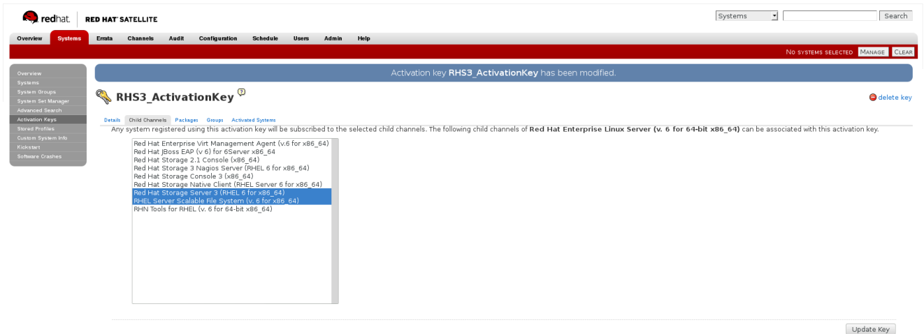
Figure 4.14. Child Channels
