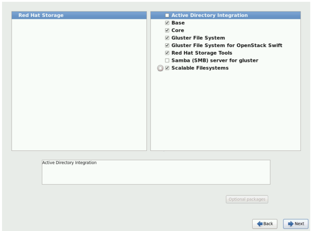
Figure 4.10. Customize Packages
