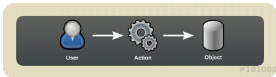
Figure 7.1. Actions
