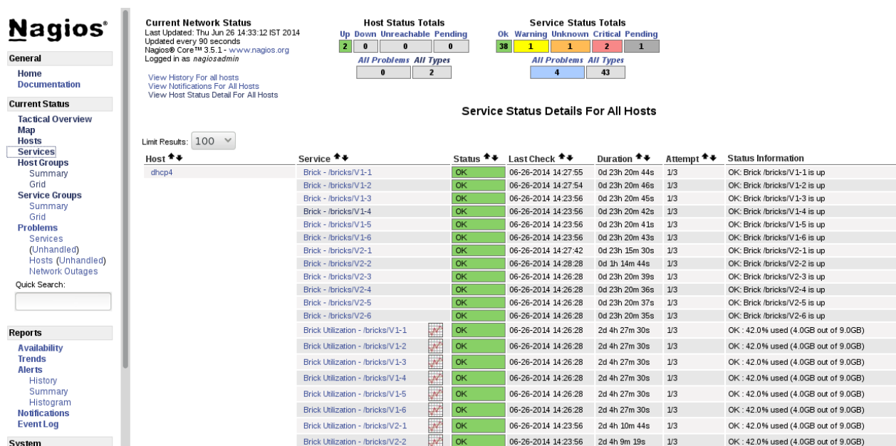
Figure 9.2. Nagios Services
