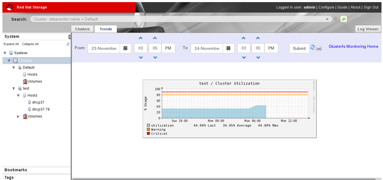
Figure 9.13. Trends
