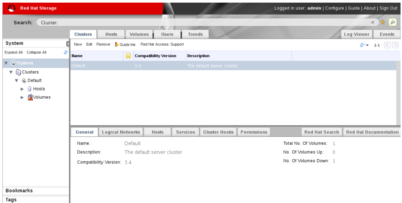
Figure 3.1. Clusters Tab
