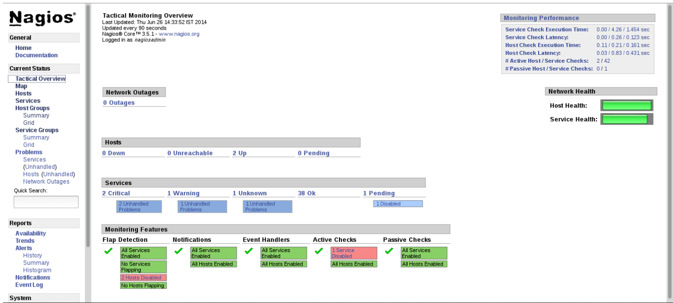
Figure 9.4. Tactical Overview
