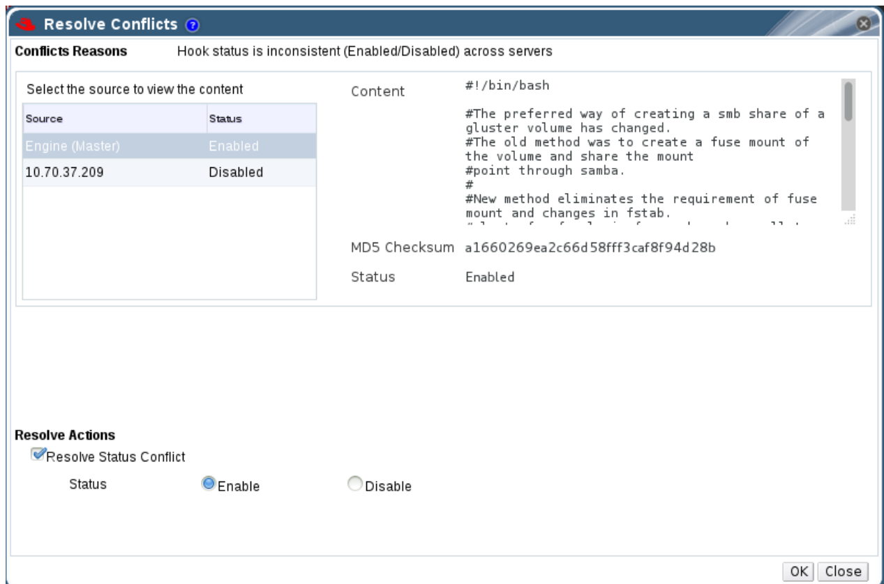
Figure 6.5. Status Conflict
