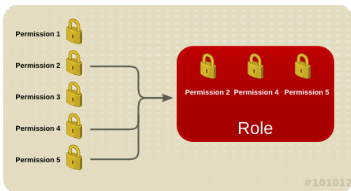
Figure 7.2. Permissions & Roles
