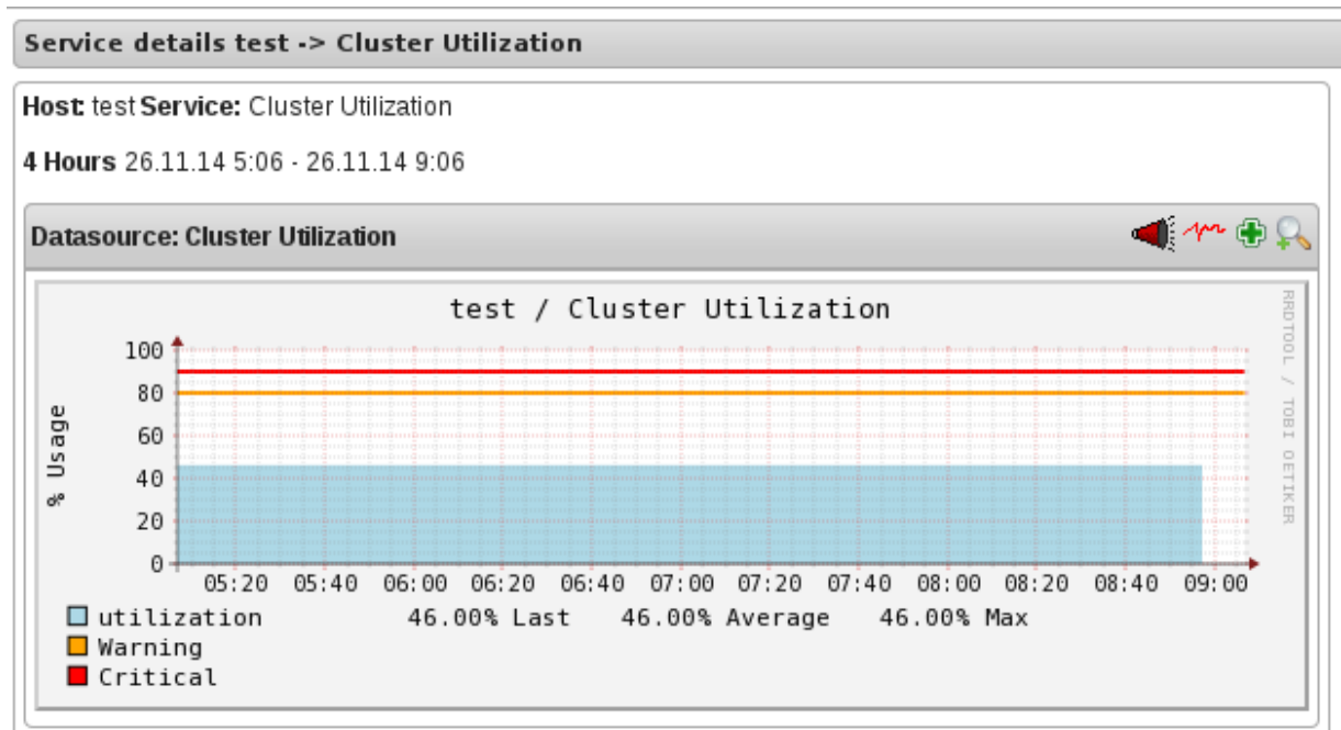
Figure 9.9. Cluster Utilization
