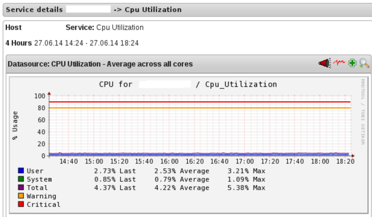
Figure 9.8. CPU Utilization
