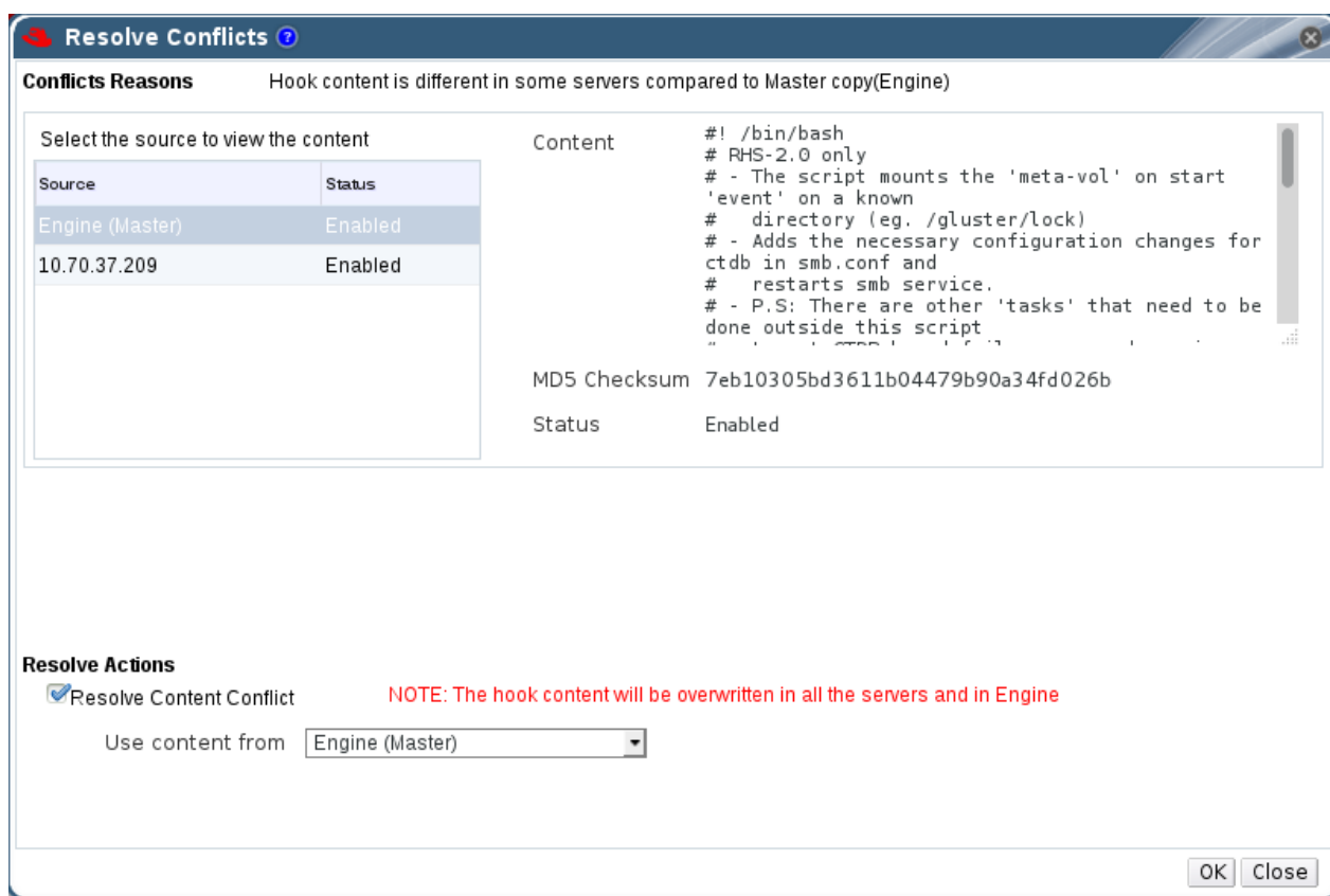
Figure 6.4. Content Conflict
