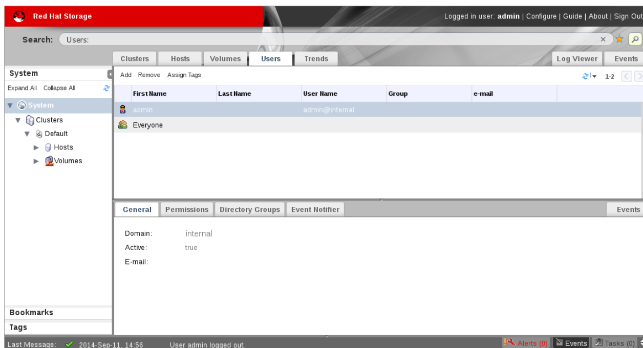
Figure 7.4. Users Tab
