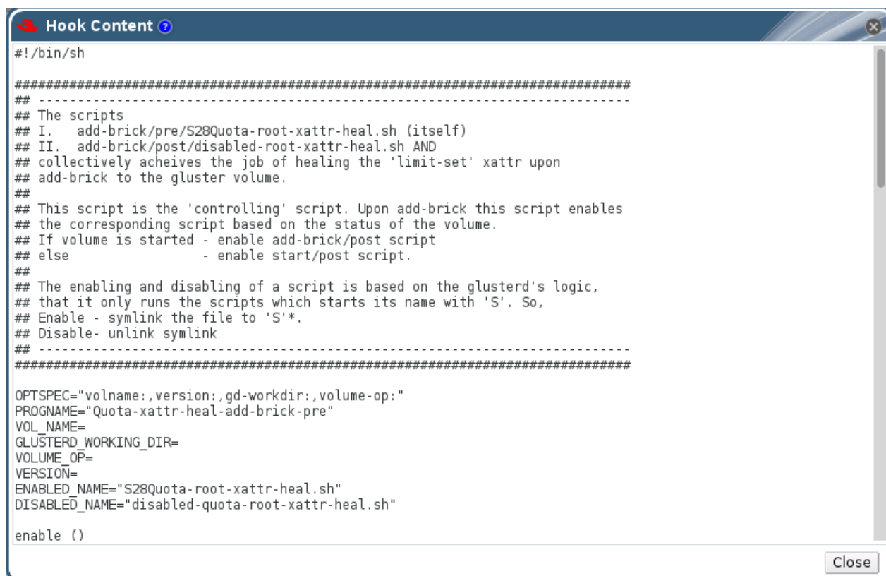
Figure 6.2. Hook Content
