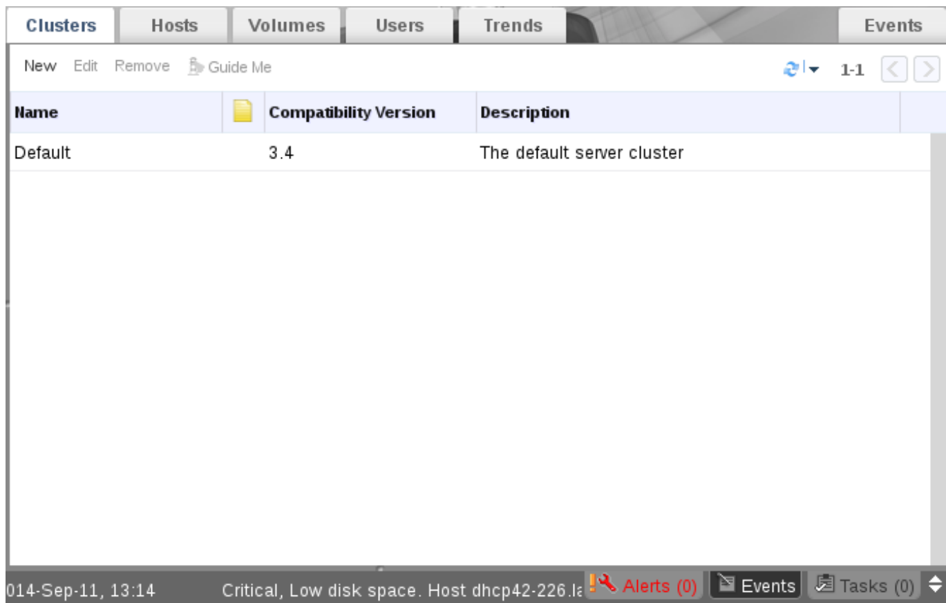
Figure 2.3. Flat Mode
