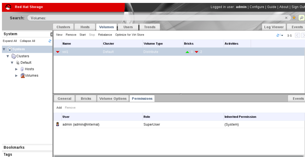
Figure 5.7. Volume Permissions
