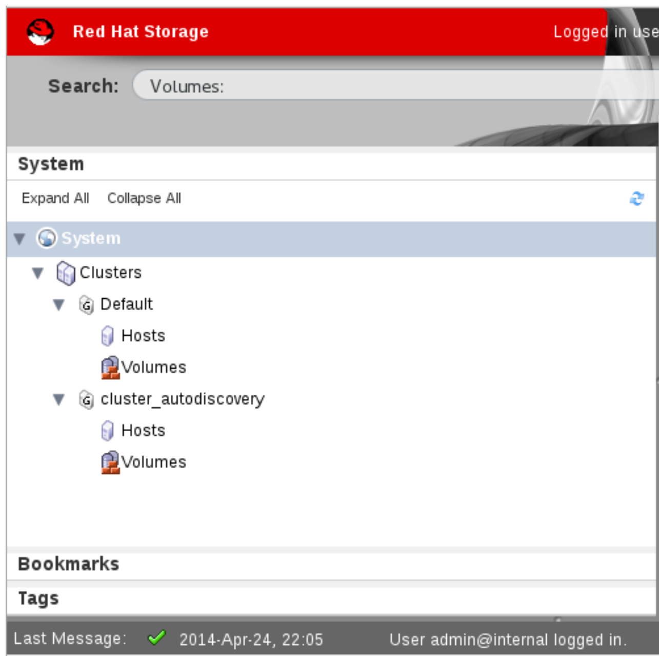
Figure 2.2. Tree Mode
