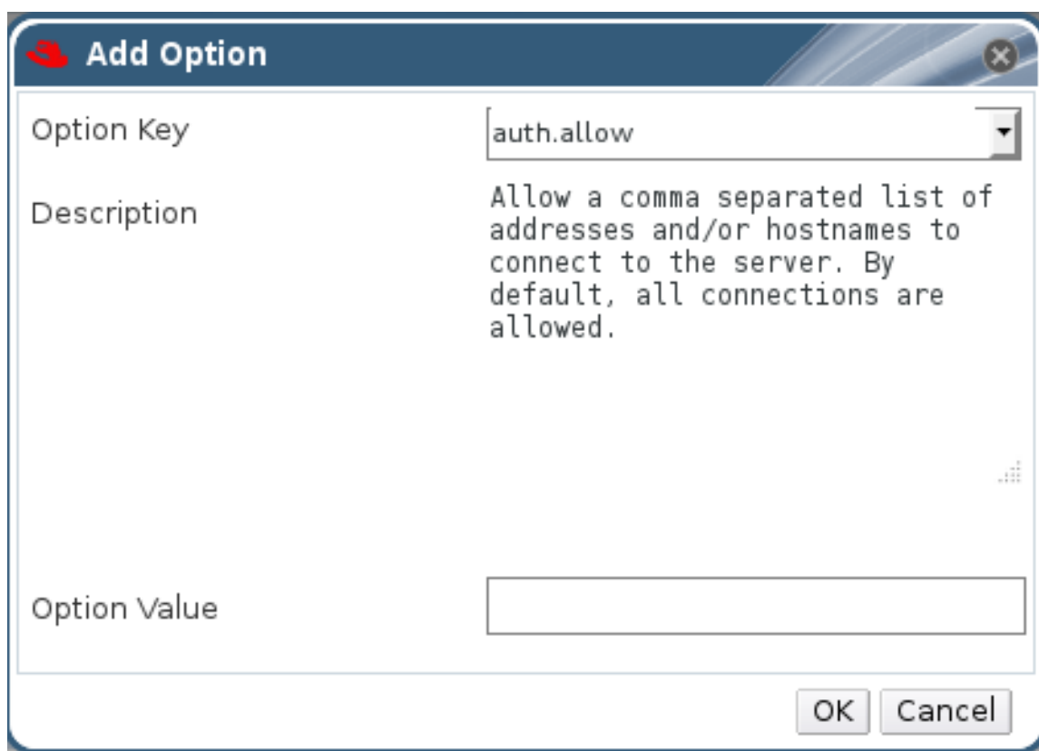
Figure 5.2. Add Option
